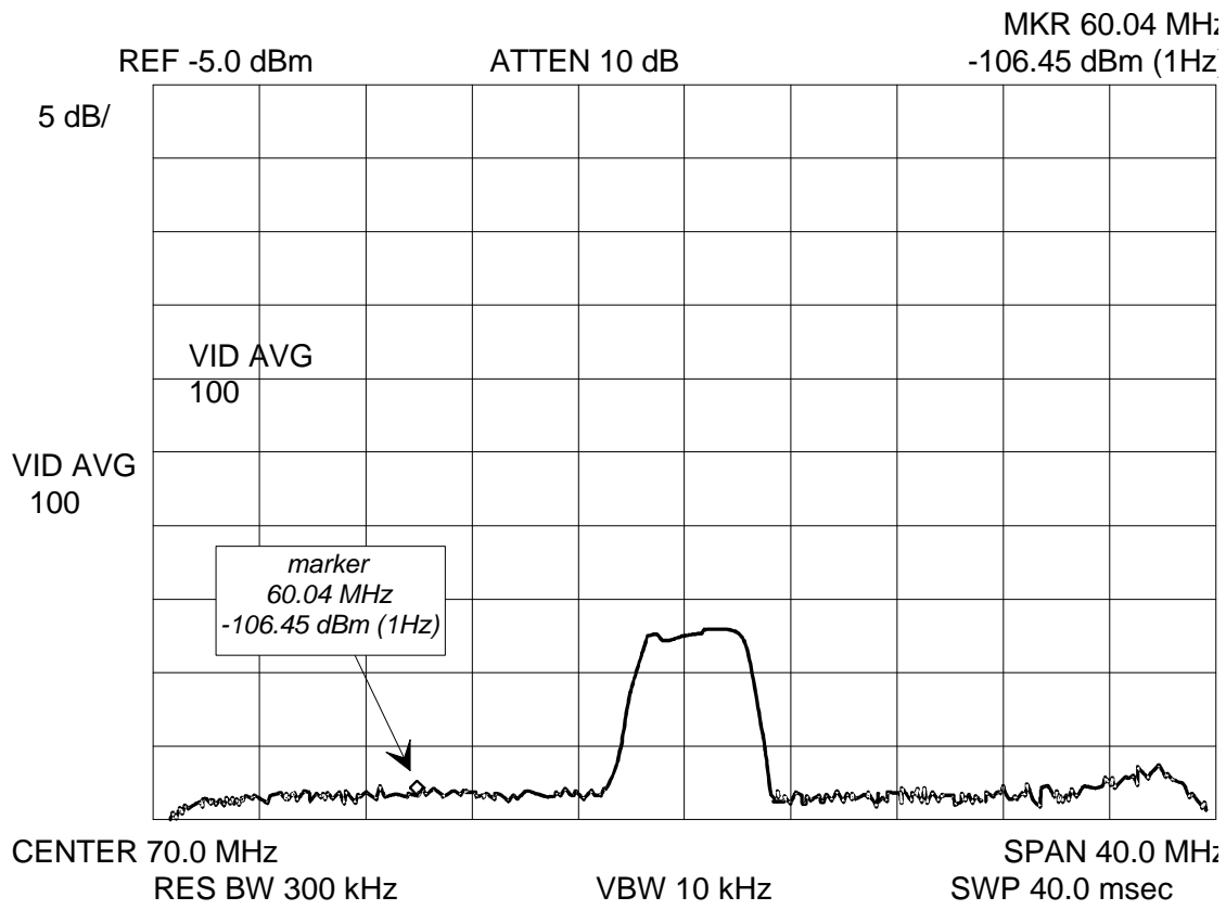
Figure 5.1.b, Measurement of Noise Power Density
